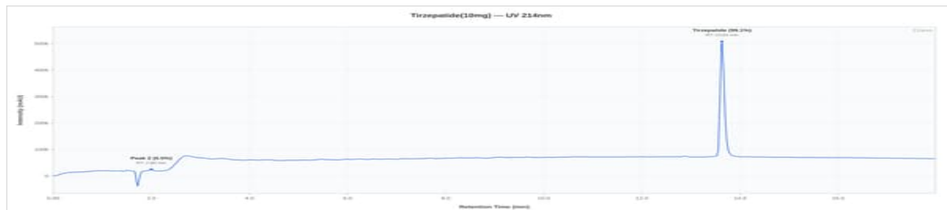
GLP-1 TR 10mg - RC2601-02: UV Chromatogram
